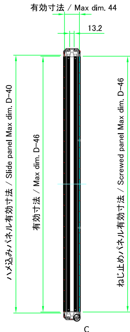
B-B (1:7)
